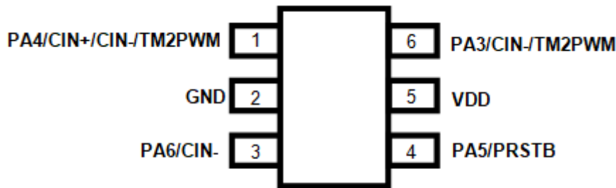
PMS150G-U06 (SOT23-6 60mil)
