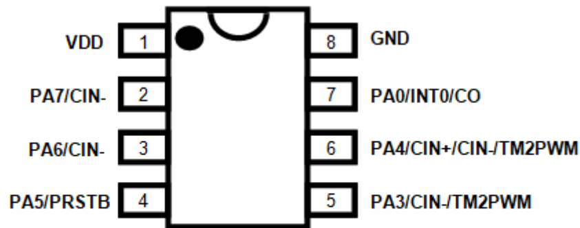
PMS150G-S08 (SOP8-150mil)
